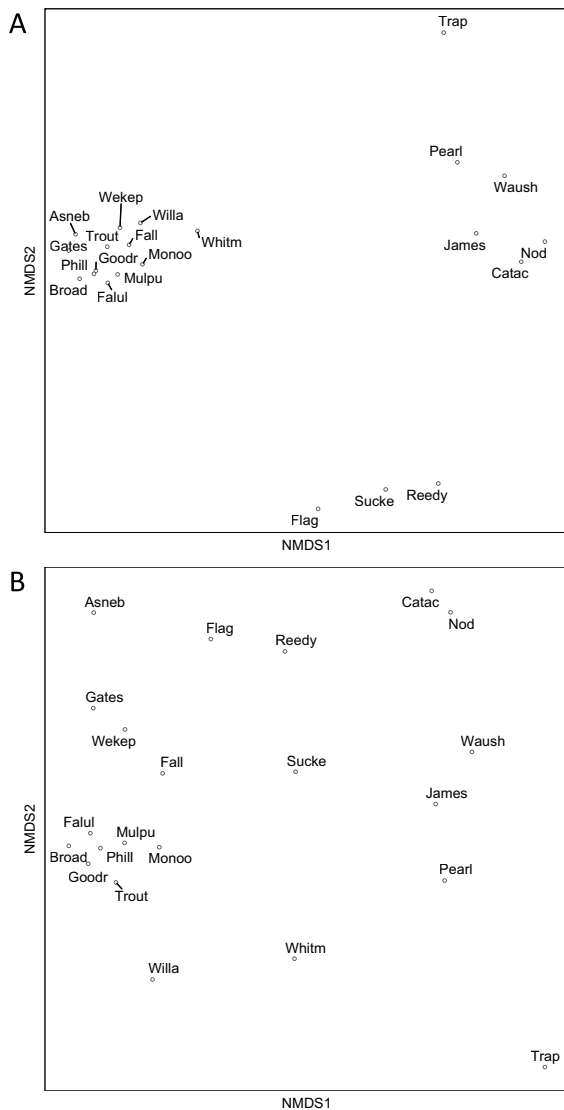
Fig. 3 NMDS ordination of species assemblage (stress = 0.08) ( A ) and trait assemblage (stress = 0.04) ( B ). Stream name abbreviations defined in Table 1, thin black lines connect text labels with sites
